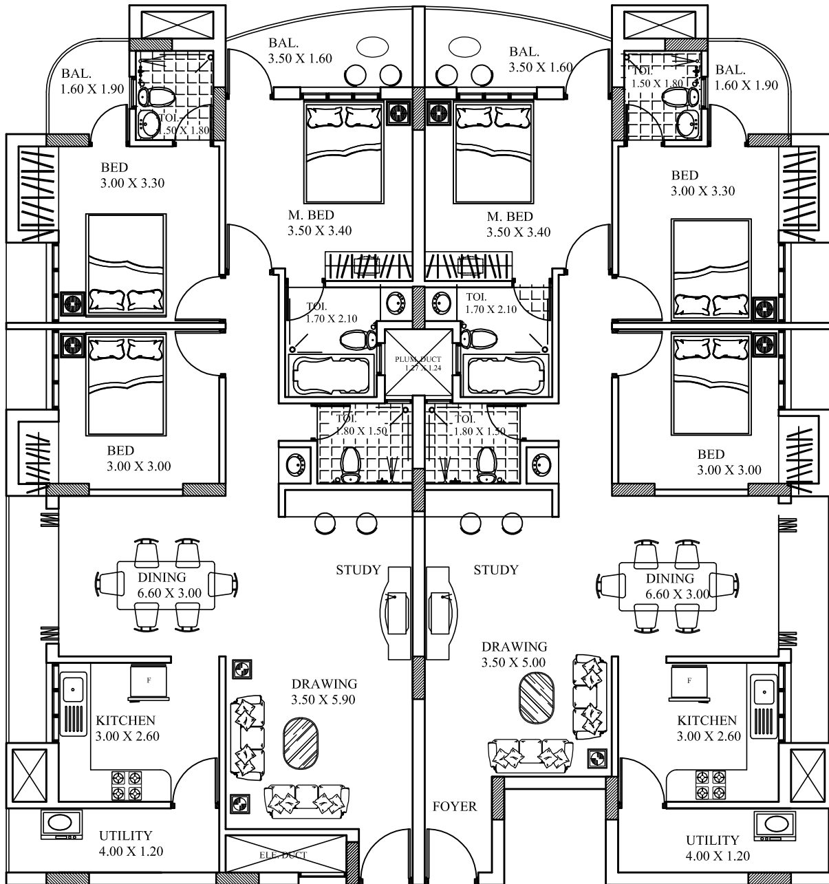
TYPICAL FLOOR PLAN 1ST TO 11 TH FLOOR
